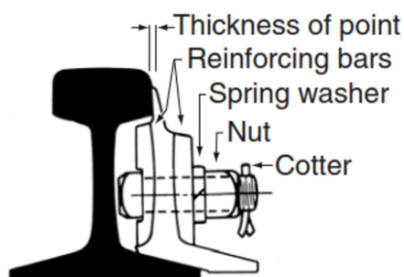
Double Reinforced Knife-Blade (Detail 6100)
